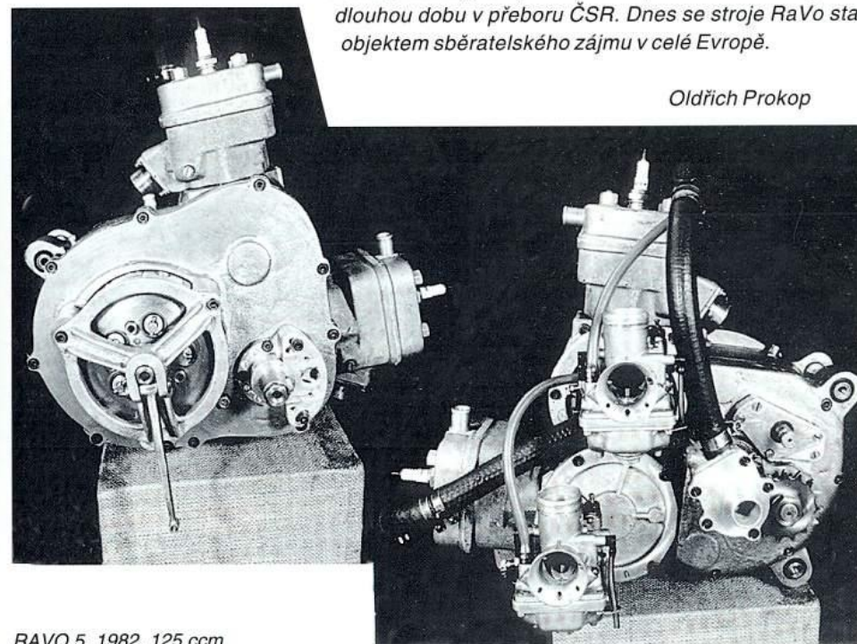
RAVO 5, 1982, 125 ccm
